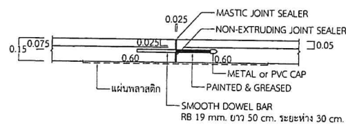
EXPANSION JOINT
