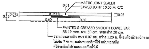
CONTRACTION JOINT
