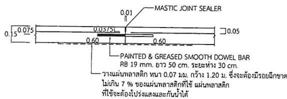
CONSTRUCTION JOINT
